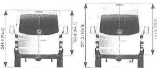
Standard Roof
